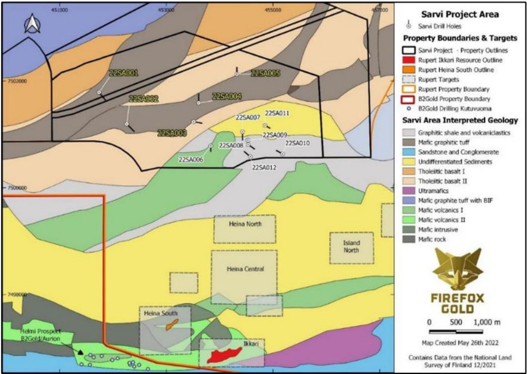
Figure 24. Initial reconnaissance drilling and interpreted geology at the Sarvi Project.
