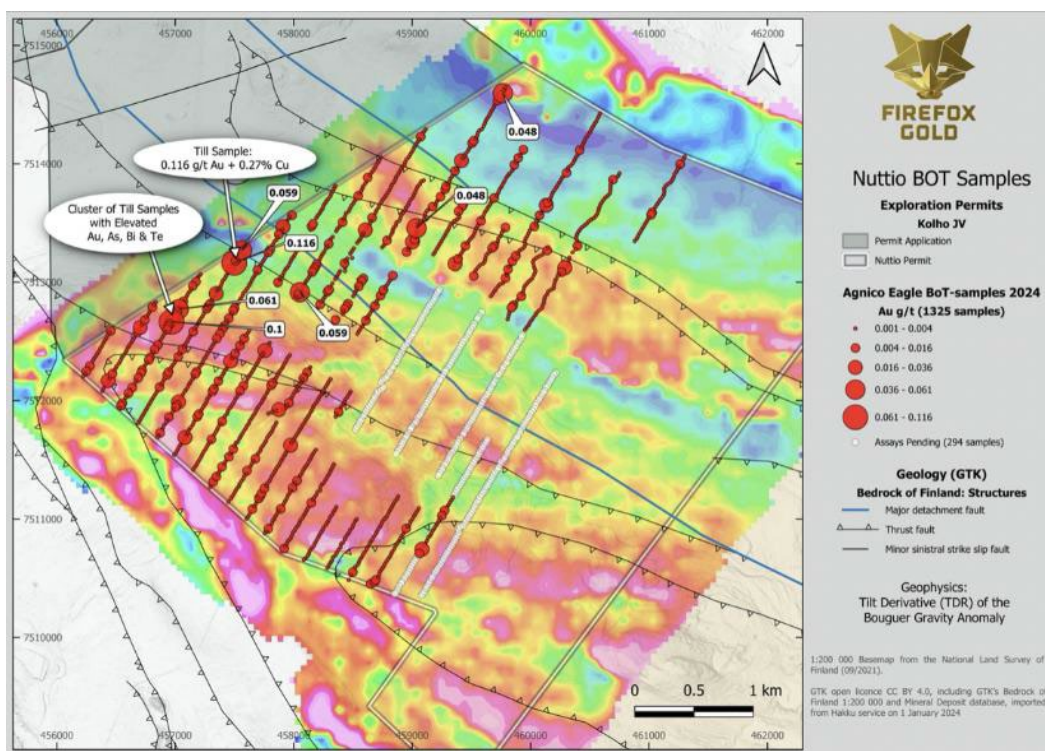
Figure 31. Gravity and gold in BoT sampling through 2024 at the Nuttio Exploration Permit (Kolho).
