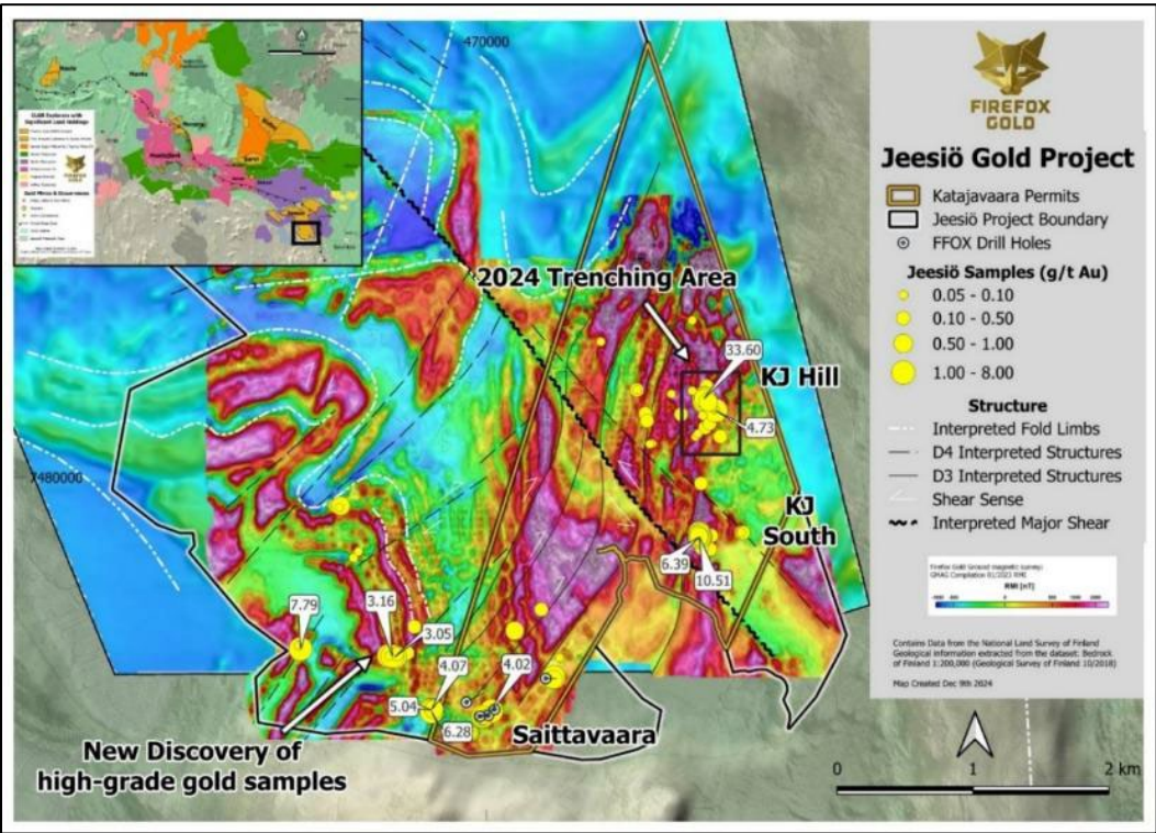
Figure 29. Magnetics interpretation and target areas in southern Jeesiö Permit.
