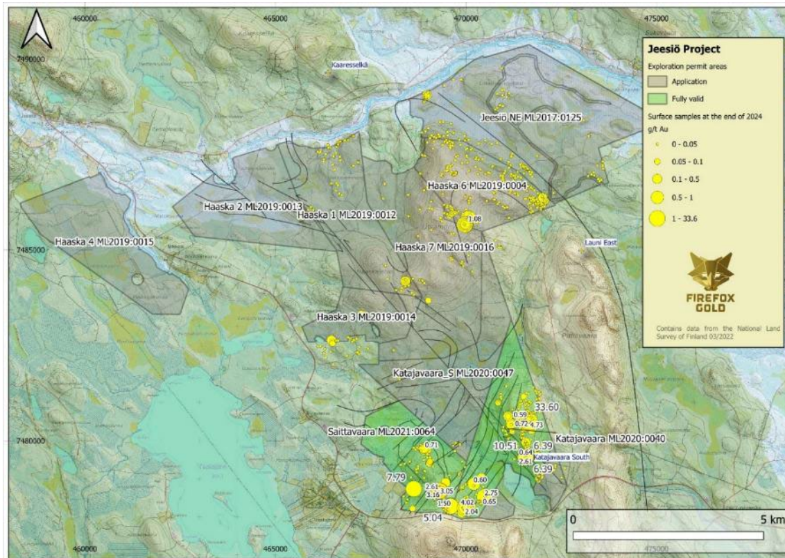
Figure 27. Jeessio property with results of gold assays on surface rock samples to the end of 2024.
