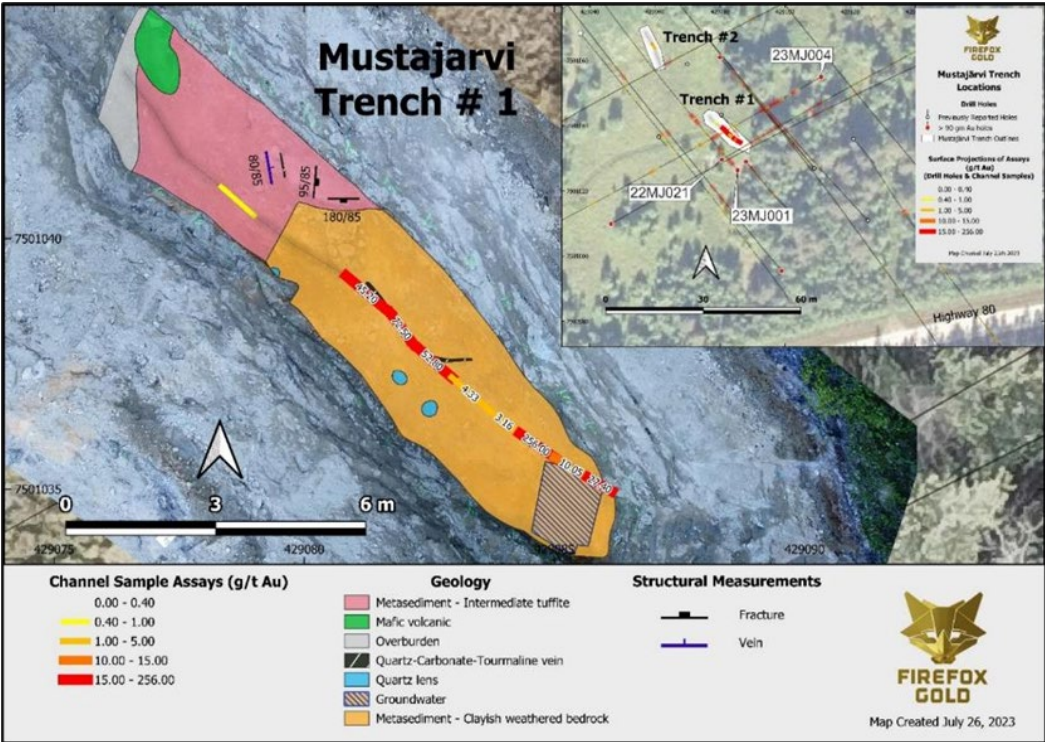
persists for hundreds of metres to the south (Figure 11).Figure 9. Mustajärvi East Zone 2023 exploration trench locations and trench 1 details.
